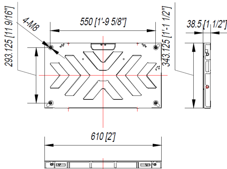
PANEL HOLE POSITION DRAWING
